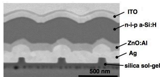
Figure 3: Cross section of cell with 340 nm thick a-Si:H after fabrication showing that the layer depositions are highly conformal.
